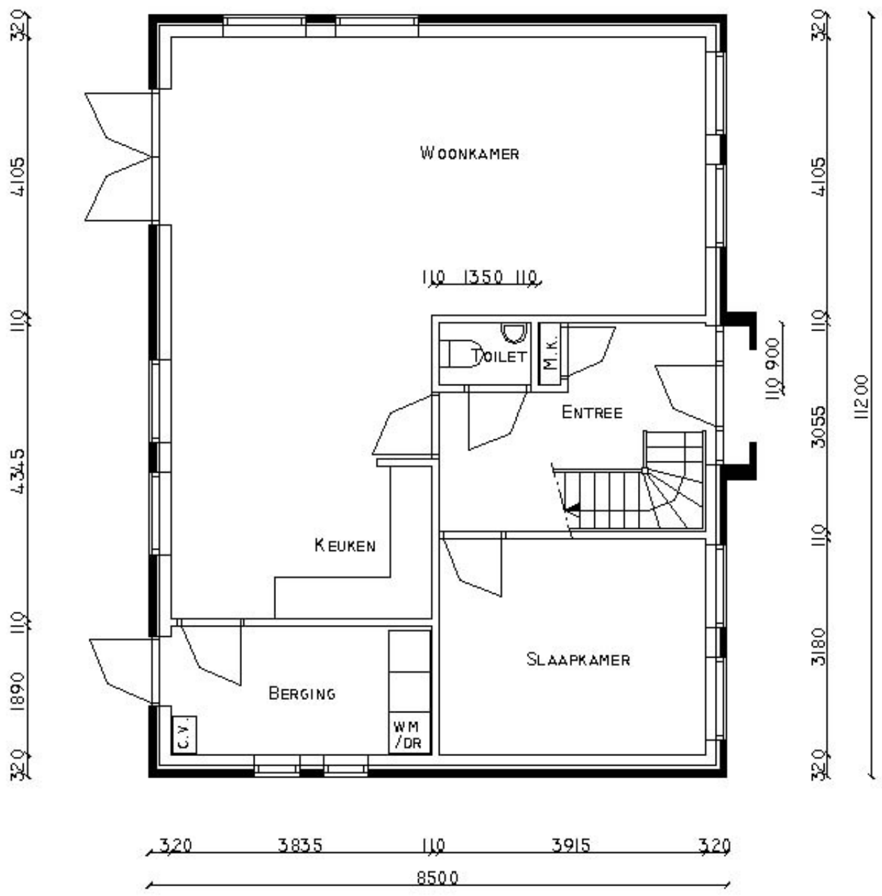
BGG. WONING 8.5 x 11.20 M TYPE HEEMSTEDÉ
