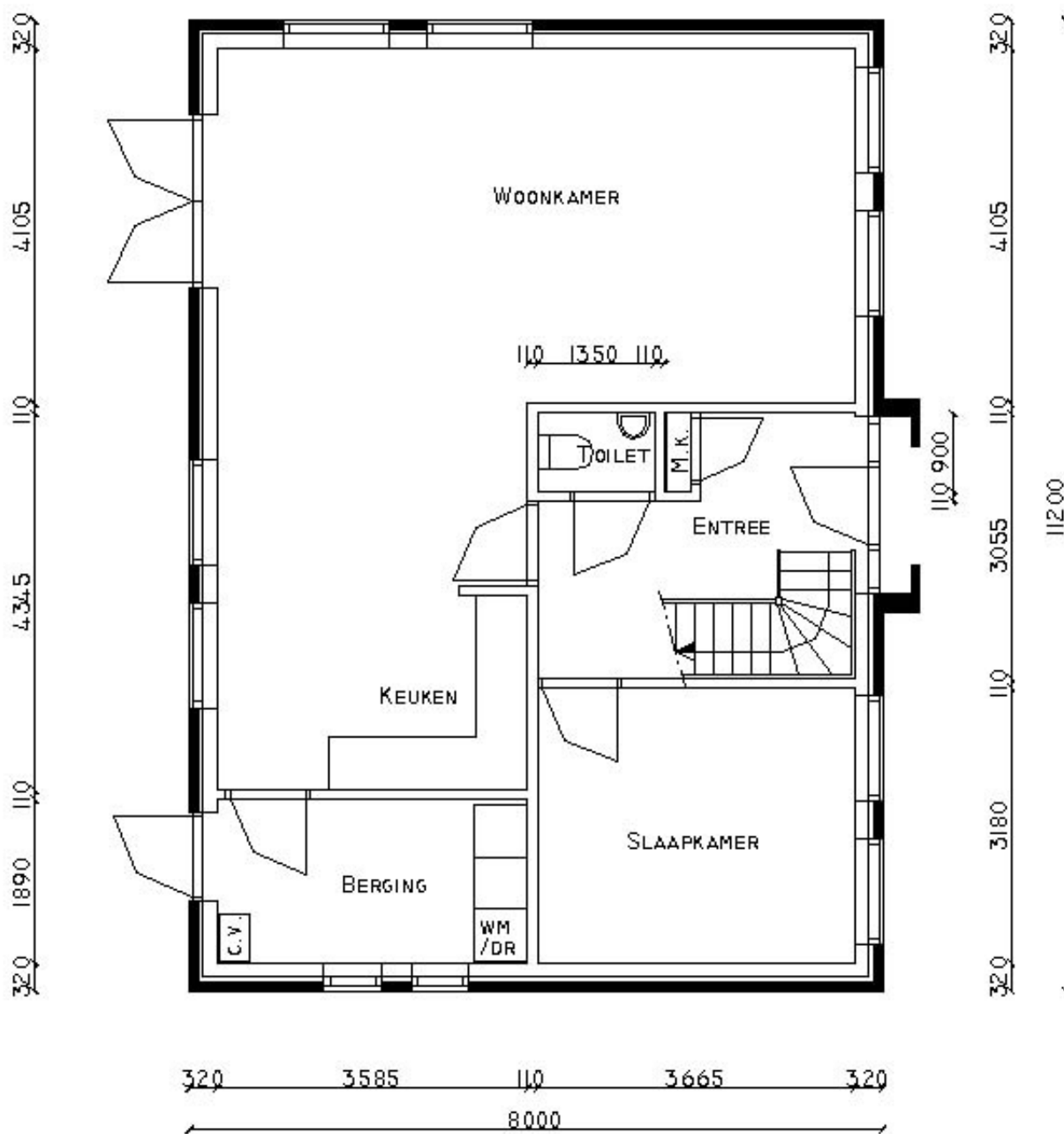
BGG. WONING 8.0 x 11.20 M TYPE HEEMSTEDE
