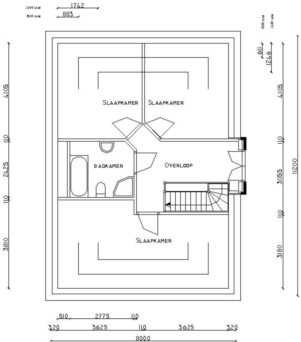
VERD. WONING 8.0 X 11.20 M TYPE HEEMSTEDÉ
